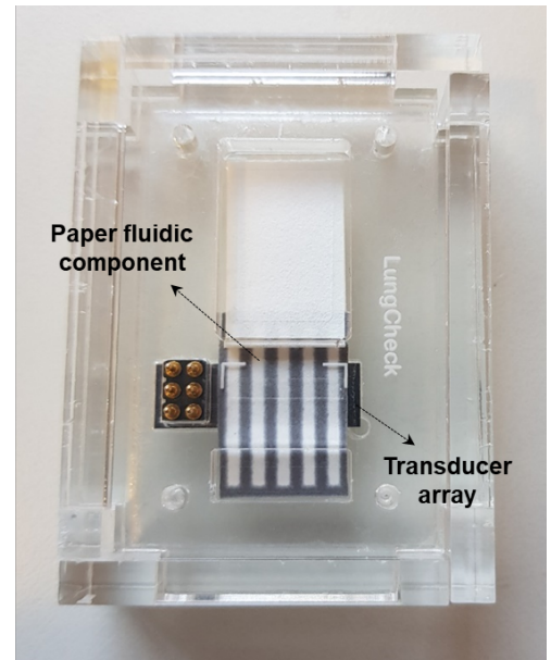
Picture of the multiplexed device prototype
